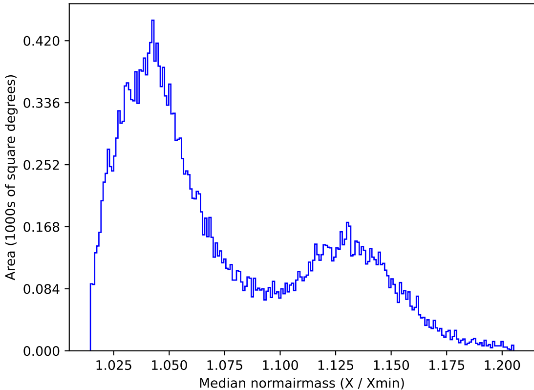
ddf_acor_sf10_lsf15_lsr20_v3.4_10yrs All sky i band: Median normairmass
