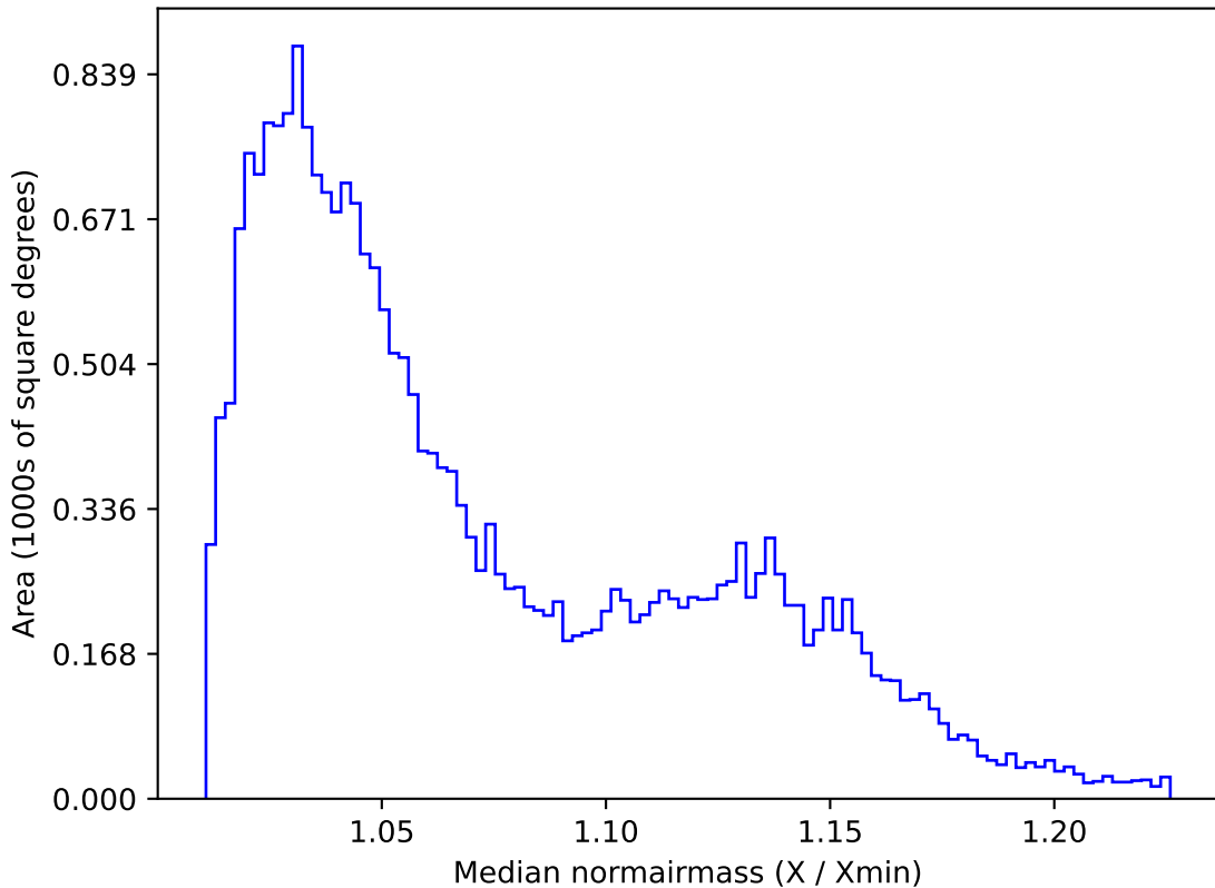
ddf_acor_sf10_lsf15_lsr20_v3.4_10yrs All sky g band: Median normairmass
