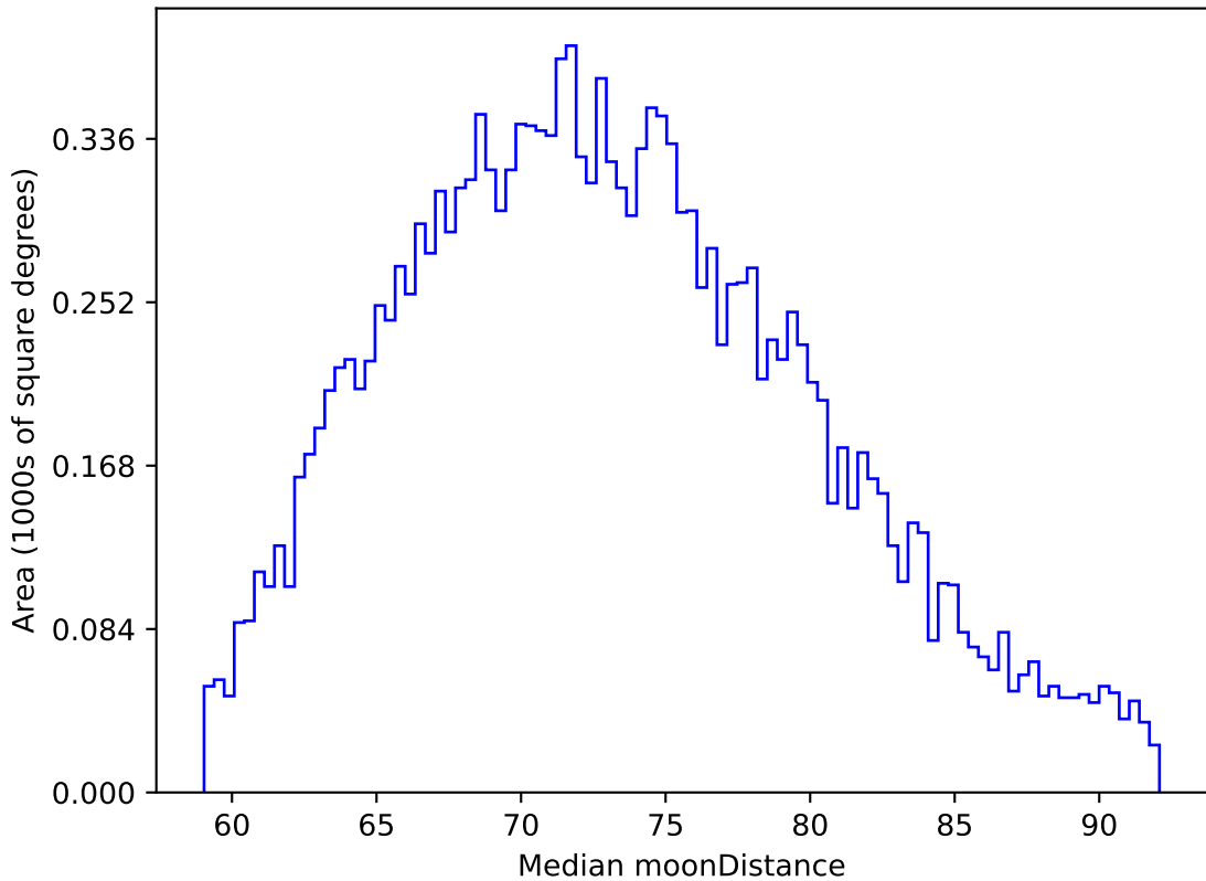
ddf_acor_sf10_lsf15_lsr20_v3.4_10yrs WFD z band: Median moonDistance
