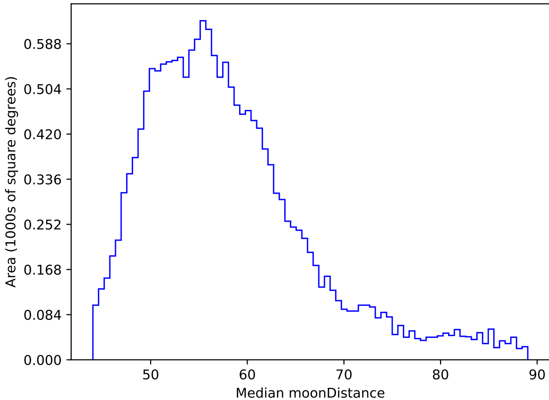
ddf_acor_sf10_lsf15_lsr20_v3.4_10yrs WFD y band: Median moonDistance
