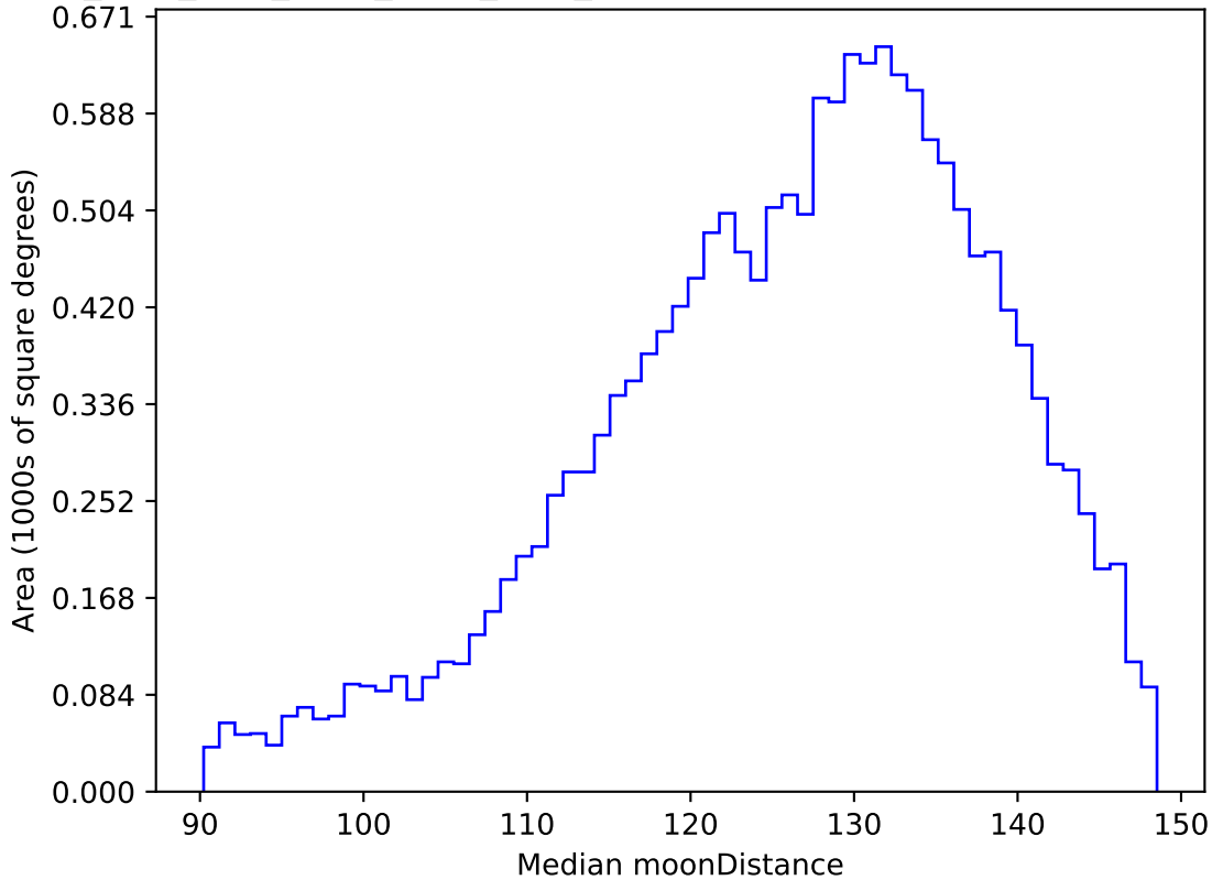
ddf_acor_sf10_lsf15_lsr20_v3.4_10yrs WFD u band: Median moonDistance
