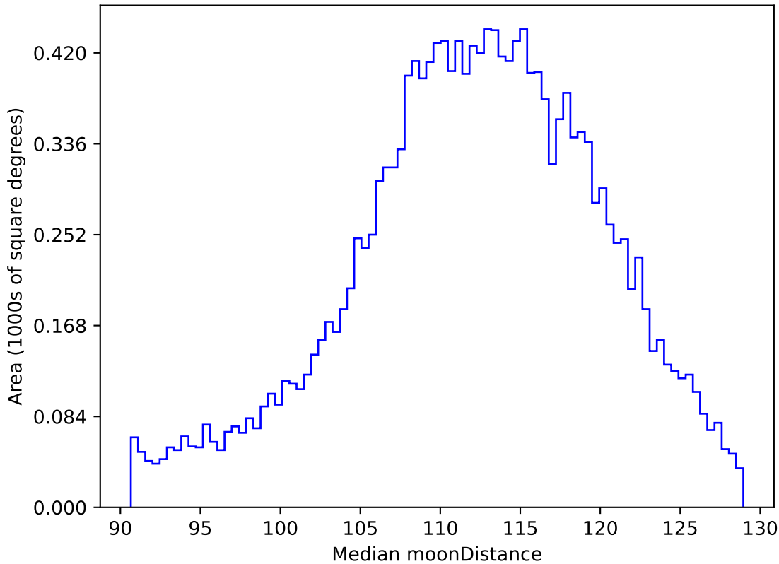
ddf_acor_sf10_lsf15_lsr20_v3.4_10yrs WFD r band: Median moonDistance
