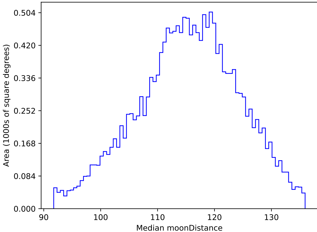
ddf_acor_sf10_ls15_lsr20_v3.4_10yrs WFD g band: Median moonDistance
