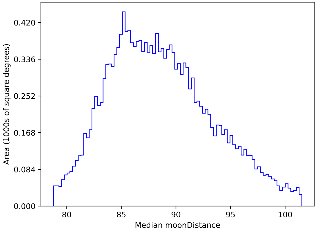
ddf_acor_sf10_lsf15_lsr20_v3.4_10yrs WFD all bands: Median moonDistance
