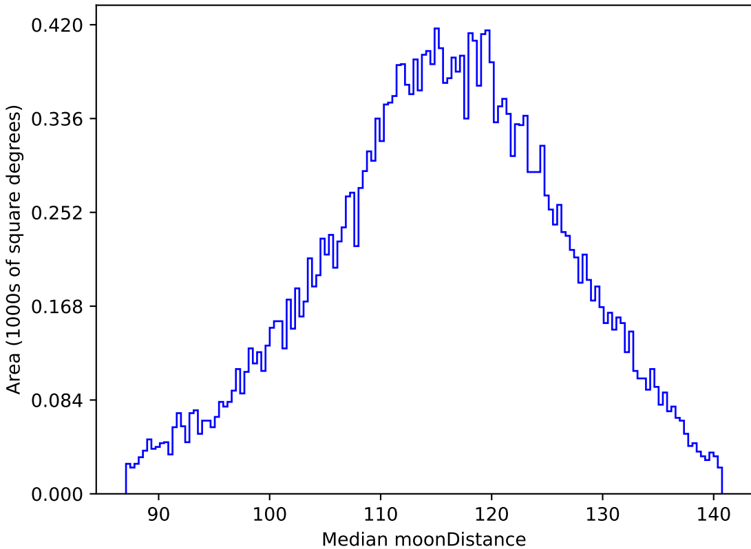
ddf_acor_sf10_lsf15_lsr20_v3.4_10yrs All sky g band: Median moonDistance
