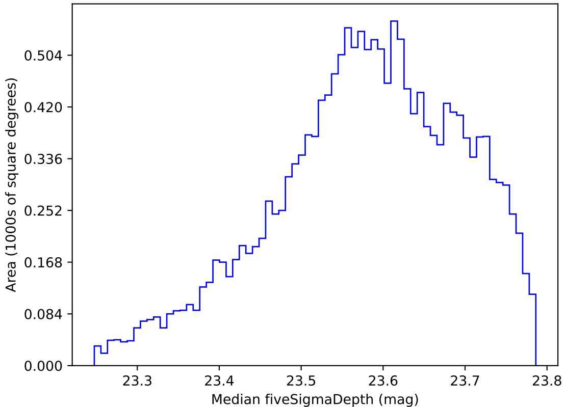
ddf_acor_sf10_lsf15_lsr20_v3.4_10yrs WFD i band: Median fiveSigmaDepth
