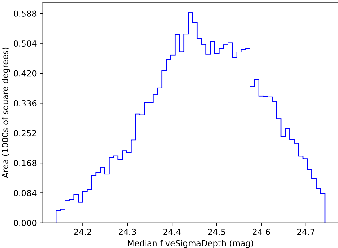
ddf_acor_sf10_lsf15_lsr20_v3.4_10yrs WFD g band: Median fiveSigmaDepth
