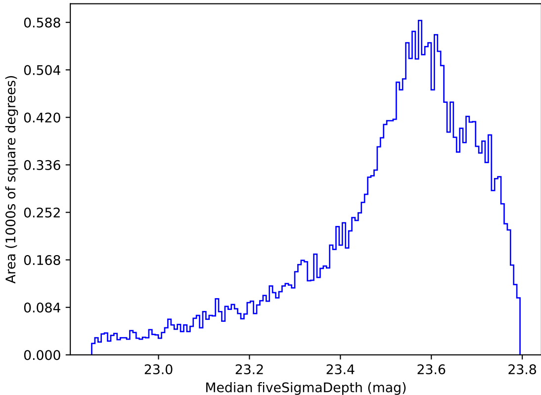
ddf_acor_sf10_lsf15_lsr20_v3.4_10yrs All sky i band: Median fiveSigmaDepth
