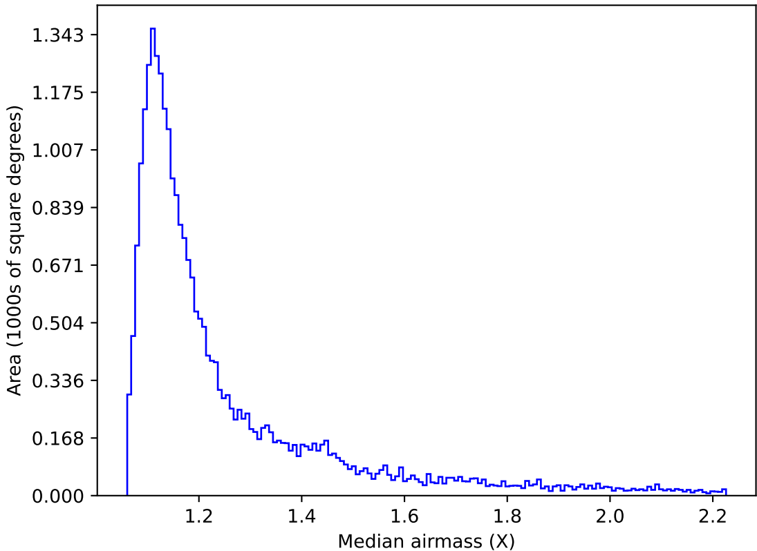
ddf_acor_sf10_lsf15_lsr20_v3.4_10yrs Yr 1 z band: Median airmass
