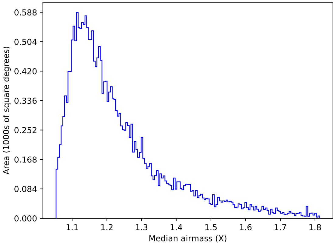
ddf_acor_sf10_lsf15_lsr20_v3.4_10yrs Yr 1 u band: Median airmass
