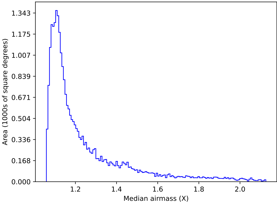
ddf_acor_sf10_lsf15_lsr20_v3.4_10yrs Yr 1 r band: Median airmass
