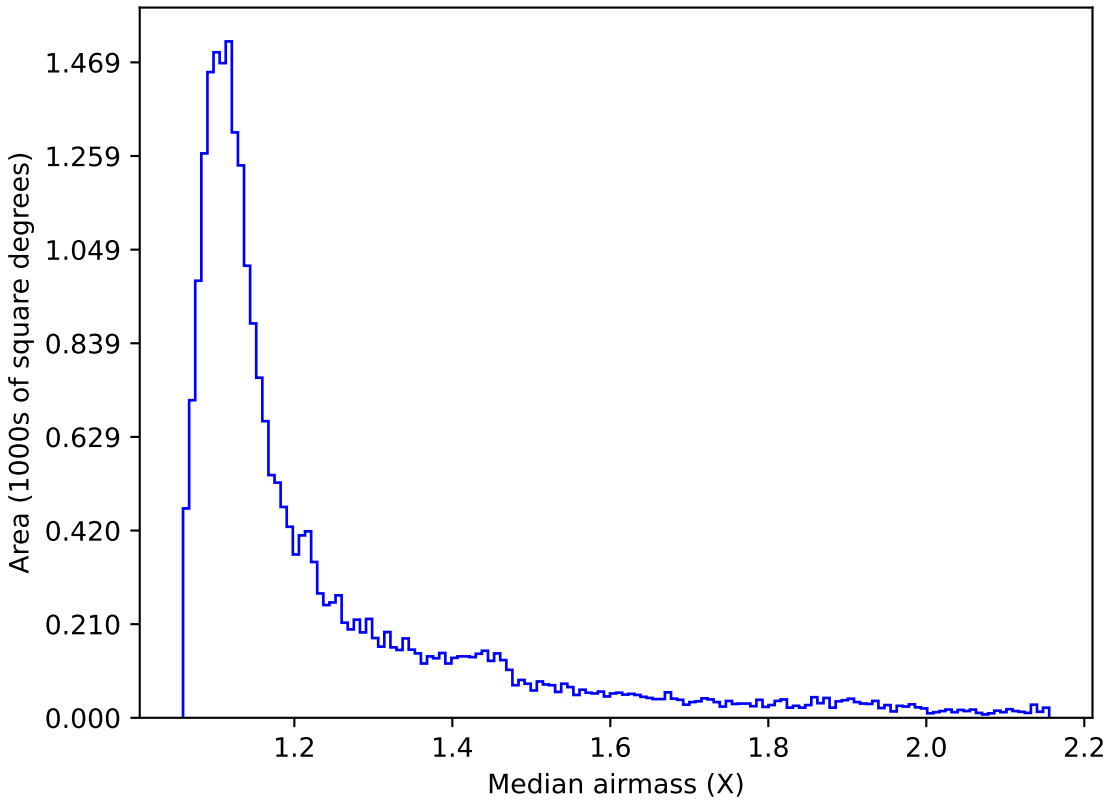
ddf_acor_sf10_lsf15_lsr20_v3.4_10yrs Yr 1 i band: Median airmass
