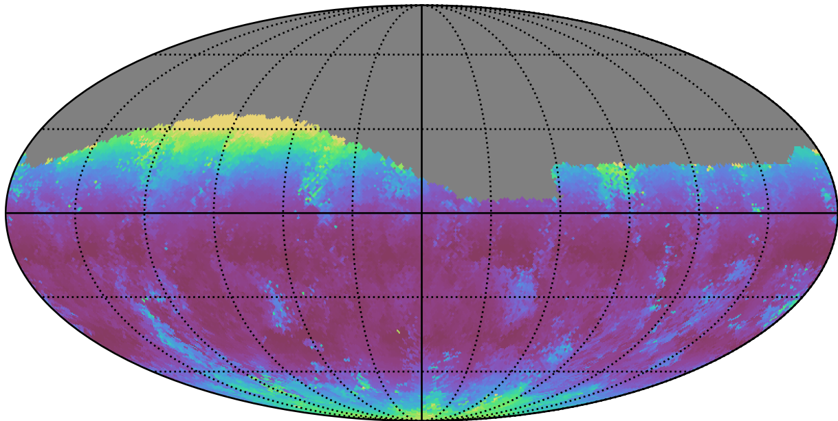
ddf_acor_sf10_lsf15_lsr20_v3.4_10yrs Yr 1 g band: Median airmass
