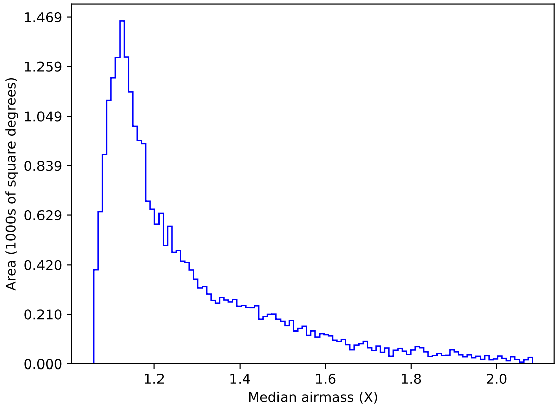
ddf_acor_sf10_lsf15_lsr20_v3.4_10yrs Yr 1 g band: Median airmass
