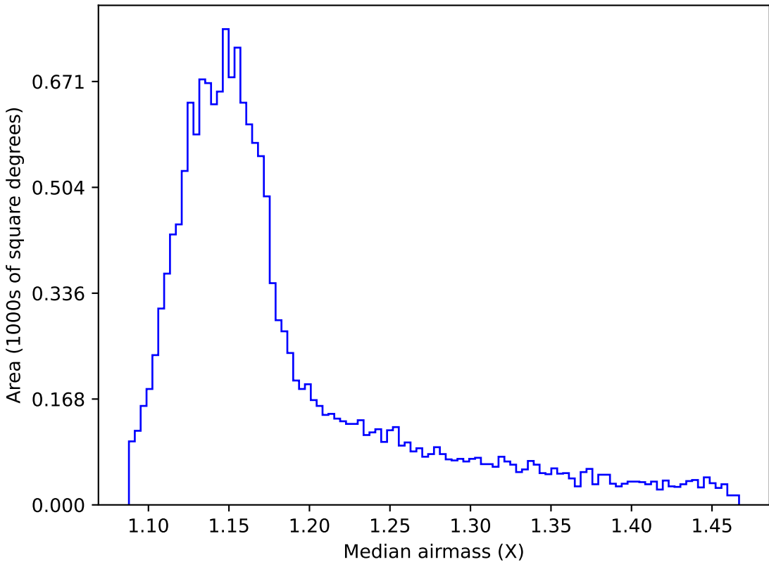
ddf_acor_sf10_ls15_lsr20_v3.4_10yrs WFD z band: Median airmass
