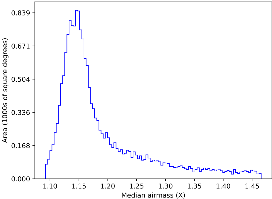
ddf_acor_sf10_ls15_lsr20_v3.4_10yrs WFD y band: Median airmass
