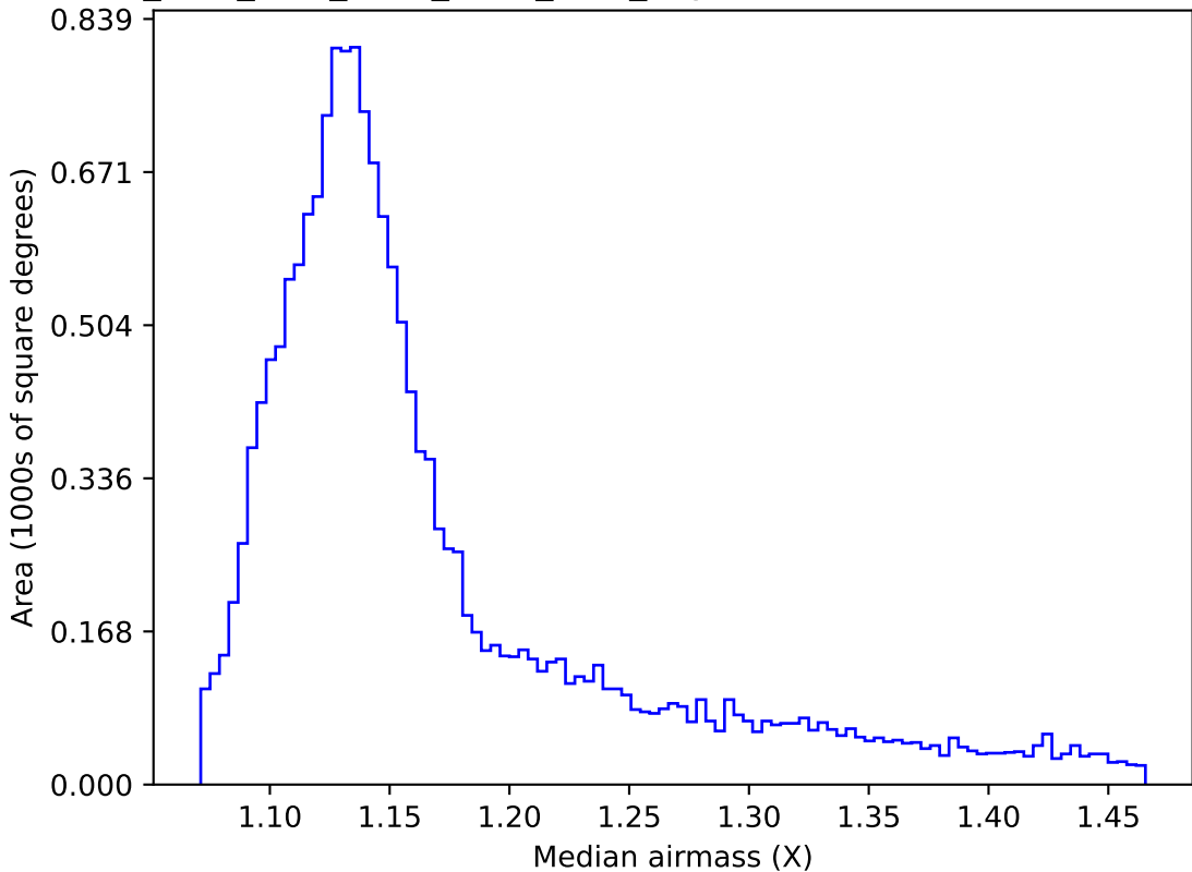
ddf_acor_sf10_lsf15_lsr20_v3.4_10yrs WFD r band: Median airmass
