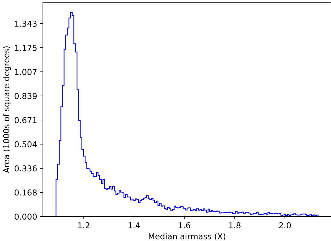
ddf_acor_sf10_lsf15_lsr20_v3.4_10yrs All sky z band: Median airmass
