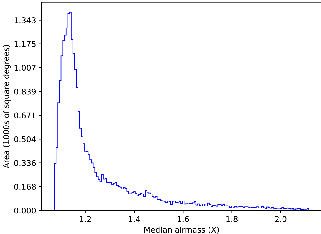
ddf_acor_sf10_lsf15_lsr20_v3.4_10yrs All sky g band: Median airmass
