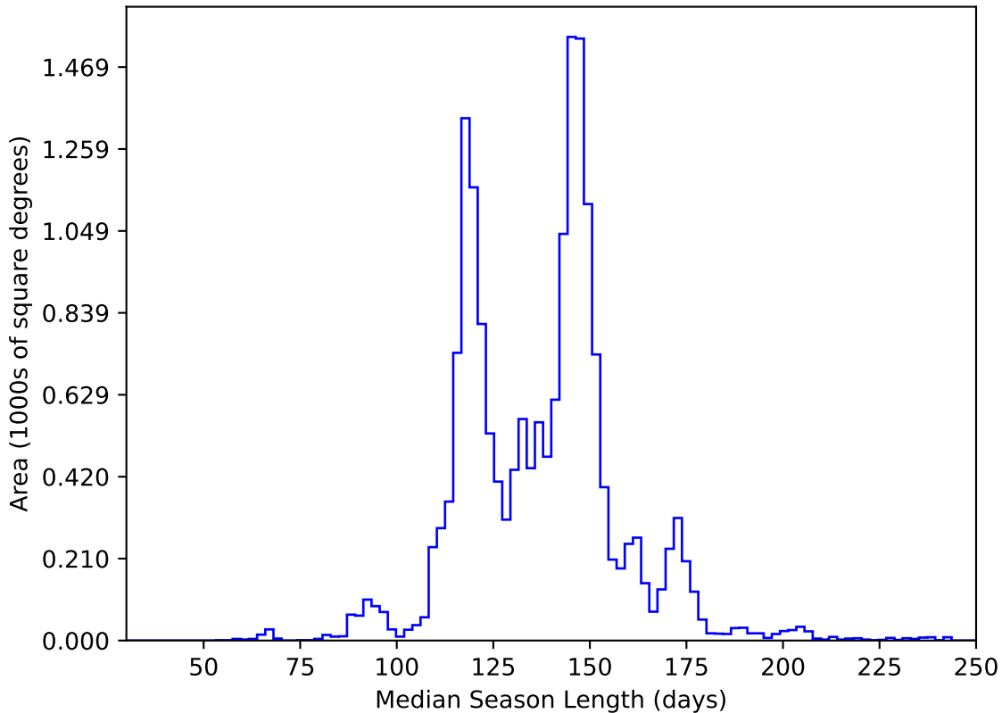
ddf_acor_sf10_lsf15_lsr20_v3.4_10yrs WFD y band: Median Season Length
