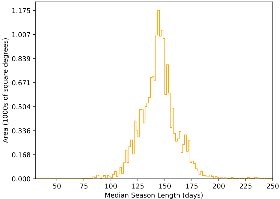
ddf_acor_sf10_lsf15_lsr20_v3.4_10yrs WFD r band: Median Season Length
