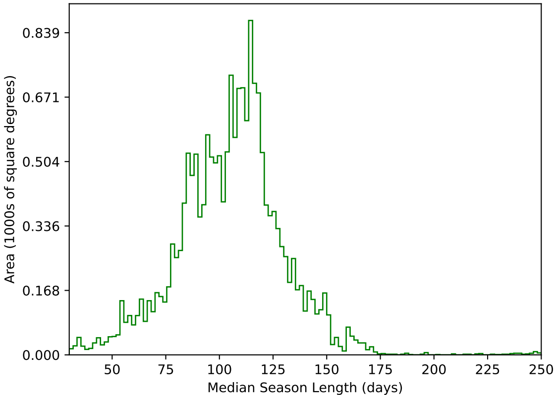
ddf_acor_sf10_ls15_lsr20_v3.4_10yrs WFD g band: Median Season Length
