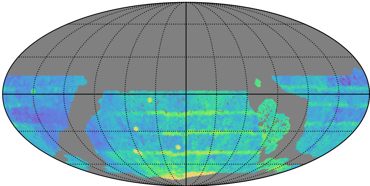
ddf_acor_sf10_lsf15_lsr20_v3.4_10yrs WFD all bands: Median Season Length
