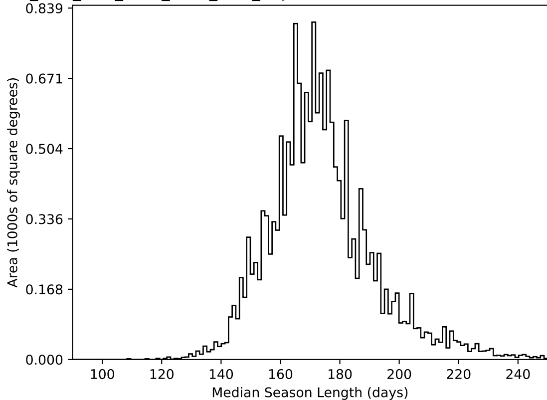
ddf_acor_sf10_lsf15_lsr20_v3.4_10yrs WFD all bands: Median Season Length
