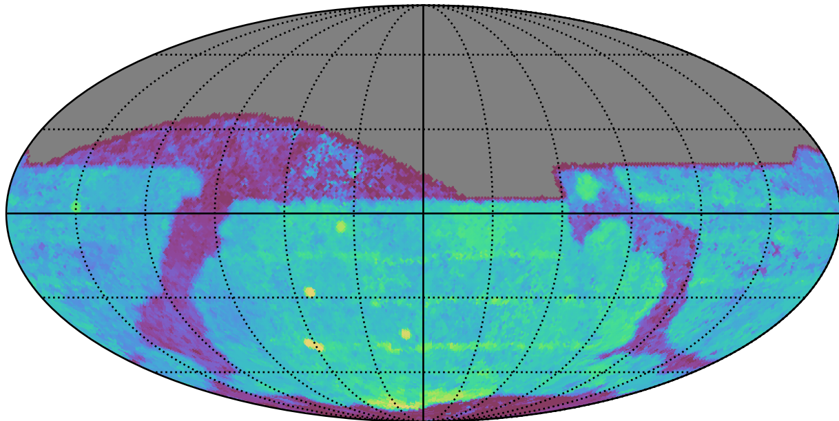
ddf_acor_sf10_lsf15_lsr20_v3.4_10yrs All sky z band: Median Season Length
