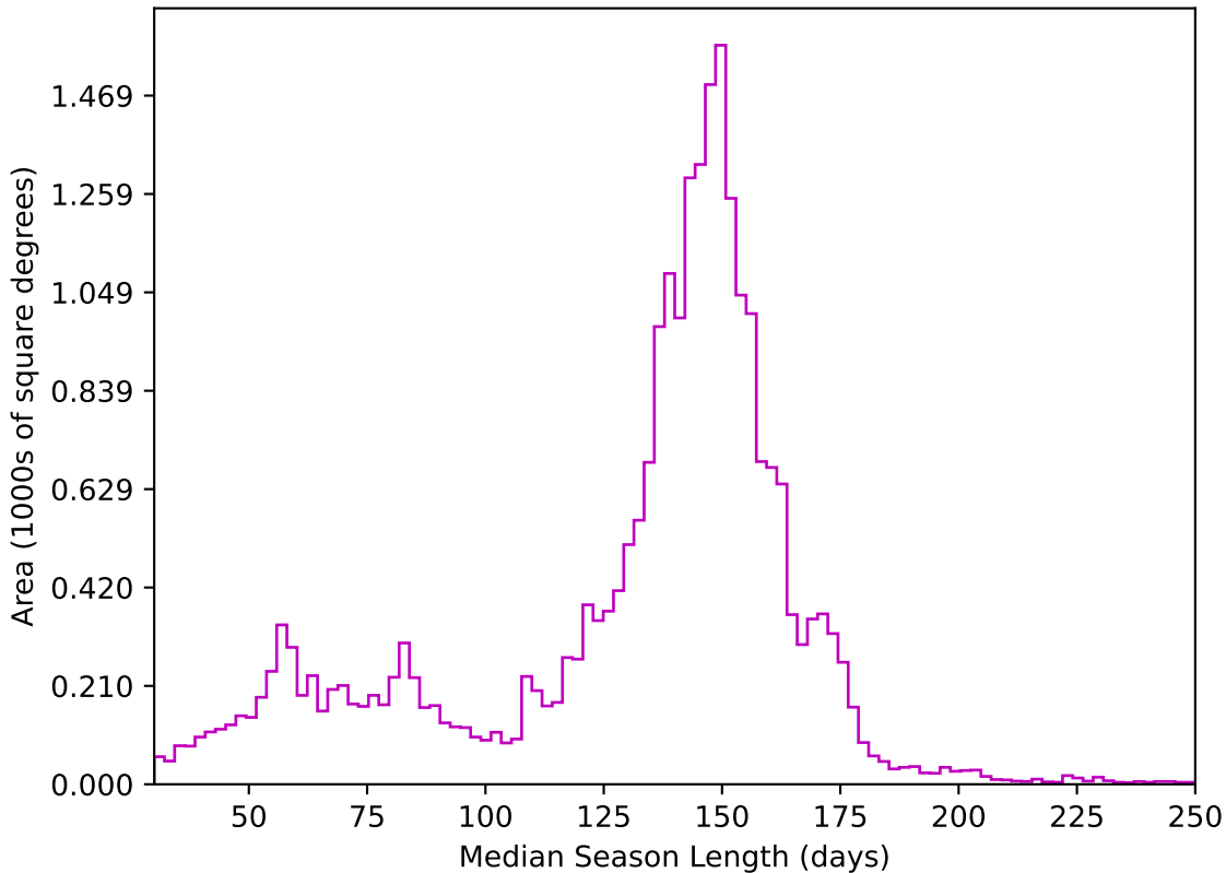
ddf_acor_sf10_lsf15_lsr20_v3.4_10yrs All sky z band: Median Season Length
