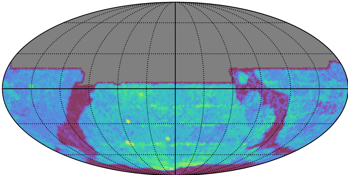
ddf_acor_sf10_lsf15_lsr20_v3.4_10yrs All sky y band: Median Season Length
