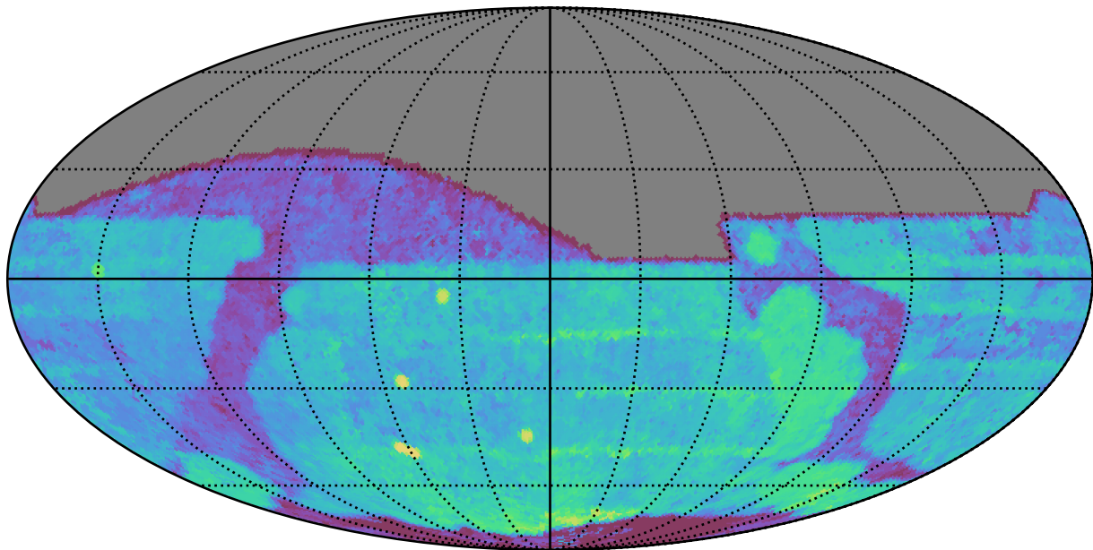
ddf_acor_sf10_lsf15_lsr20_v3.4_10yrs All sky r band: Median Season Length
