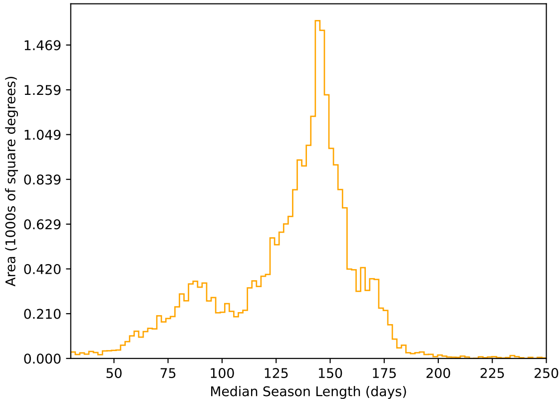
ddf_acor_sf10_lsf15_lsr20_v3.4_10yrs All sky r band: Median Season Length
