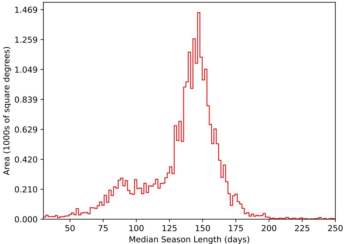
ddf_acor_sf10_lsf15_lsr20_v3.4_10yrs All sky i band: Median Season Length
