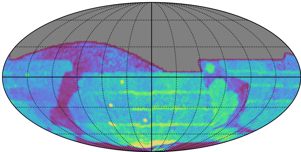
ddf_acor_sf10_lsf15_lsr20_v3.4_10yrs All sky all bands: Median Season Length
