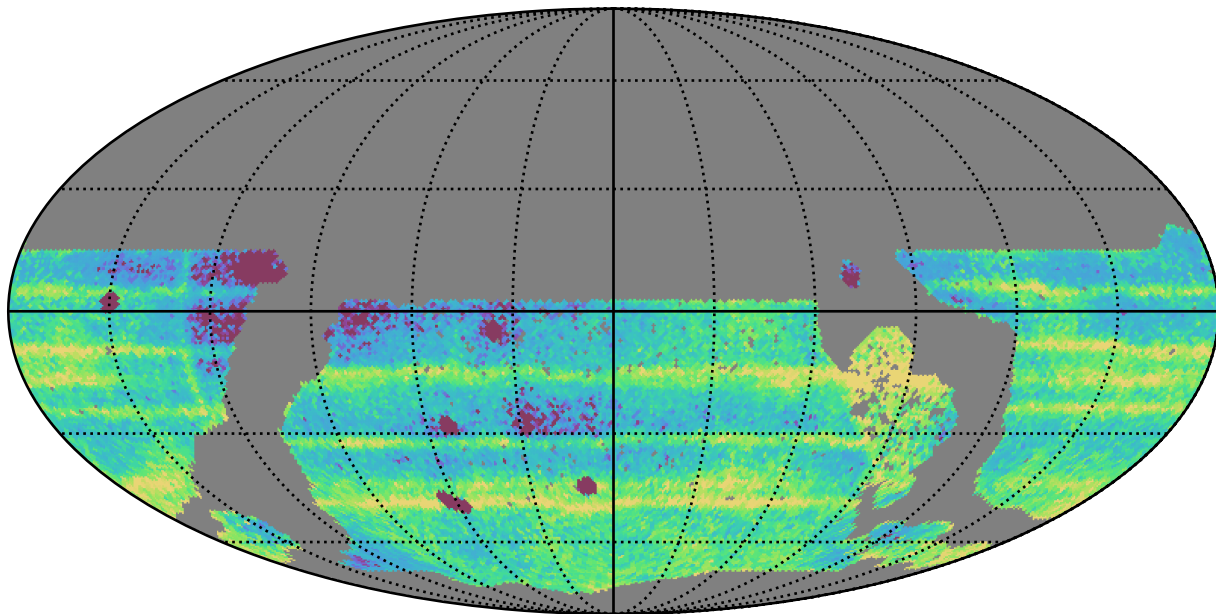
ddf_acor_sf10_lsf15_lsr20_v3.4_10yrs WFD: Median Intra-Night Gap
