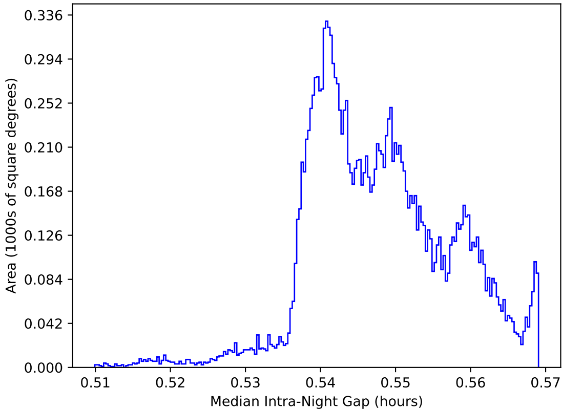
ddf_acor_sf10_lsf15_lsr20_v3.4_10yrs WFD: Median Intra-Night Gap
