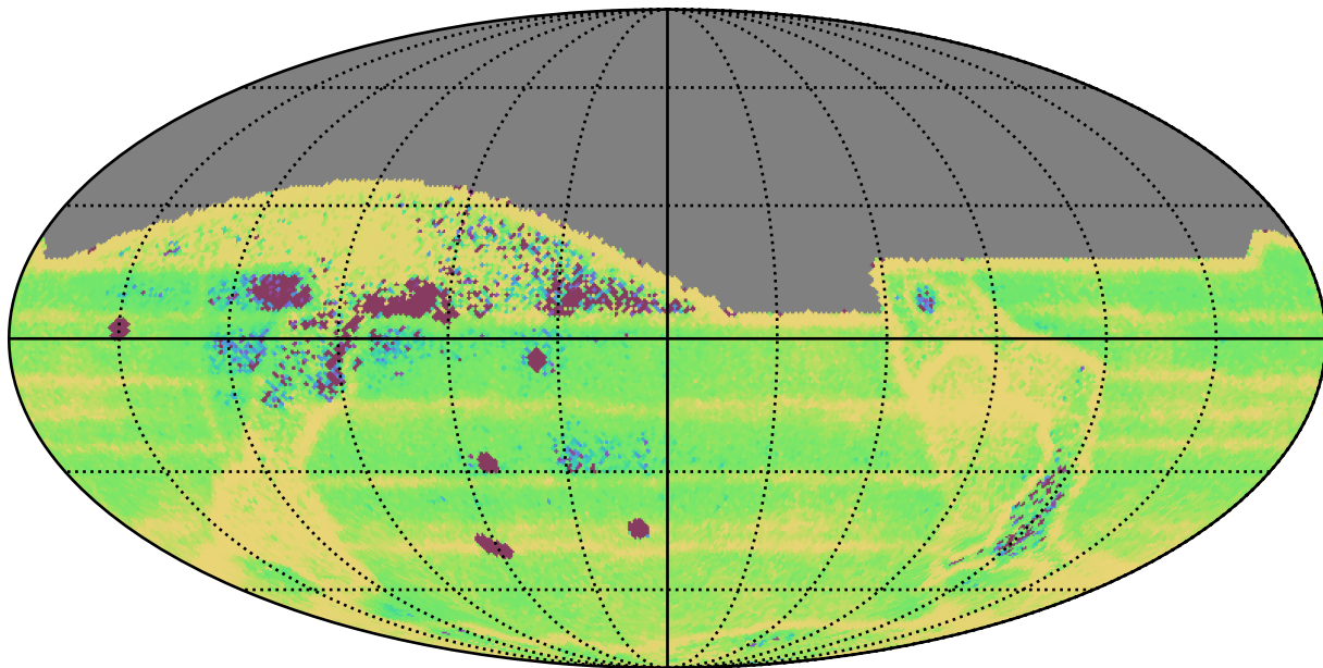
ddf_acor_sf10_lsf15_lsr20_v3.4_10yrs All sky: Median Intra-Night Gap
