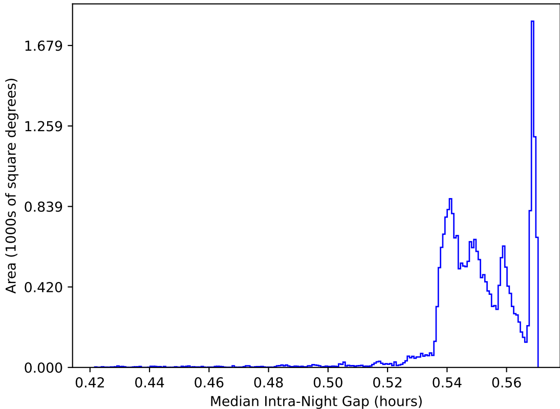
ddf_acor_sf10_lsf15_lsr20_v3.4_10yrs All sky: Median Intra-Night Gap
