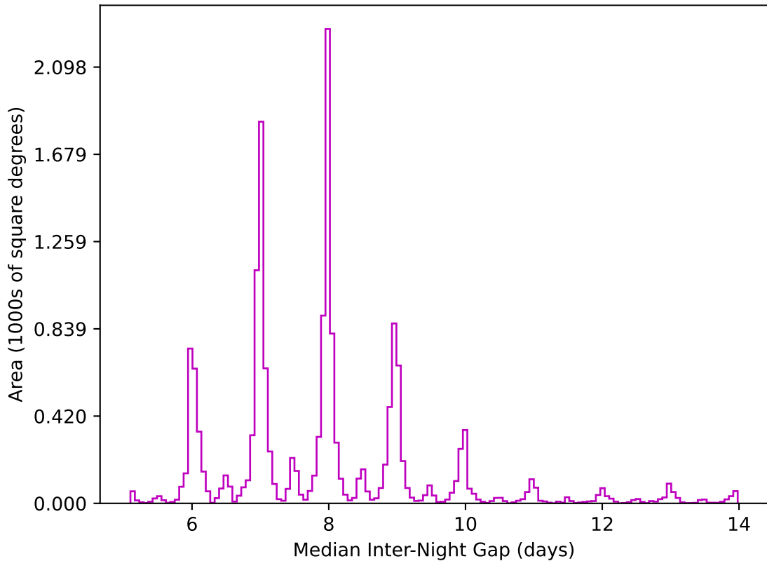
ddf_acor_sf10_lsf15_lsr20_v3.4_10yrs WFD z band: Median Inter-Night Gap
