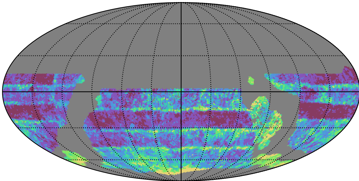
ddf_acor_sf10_lsf15_lsr20_v3.4_10yrs WFD r band: Median Inter-Night Gap
