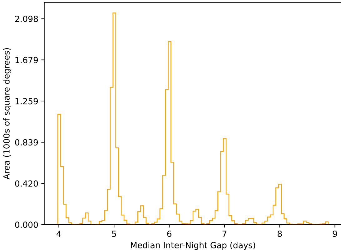
ddf_acor_sf10_lsf15_lsr20_v3.4_10yrs WFD r band: Median Inter-Night Gap
