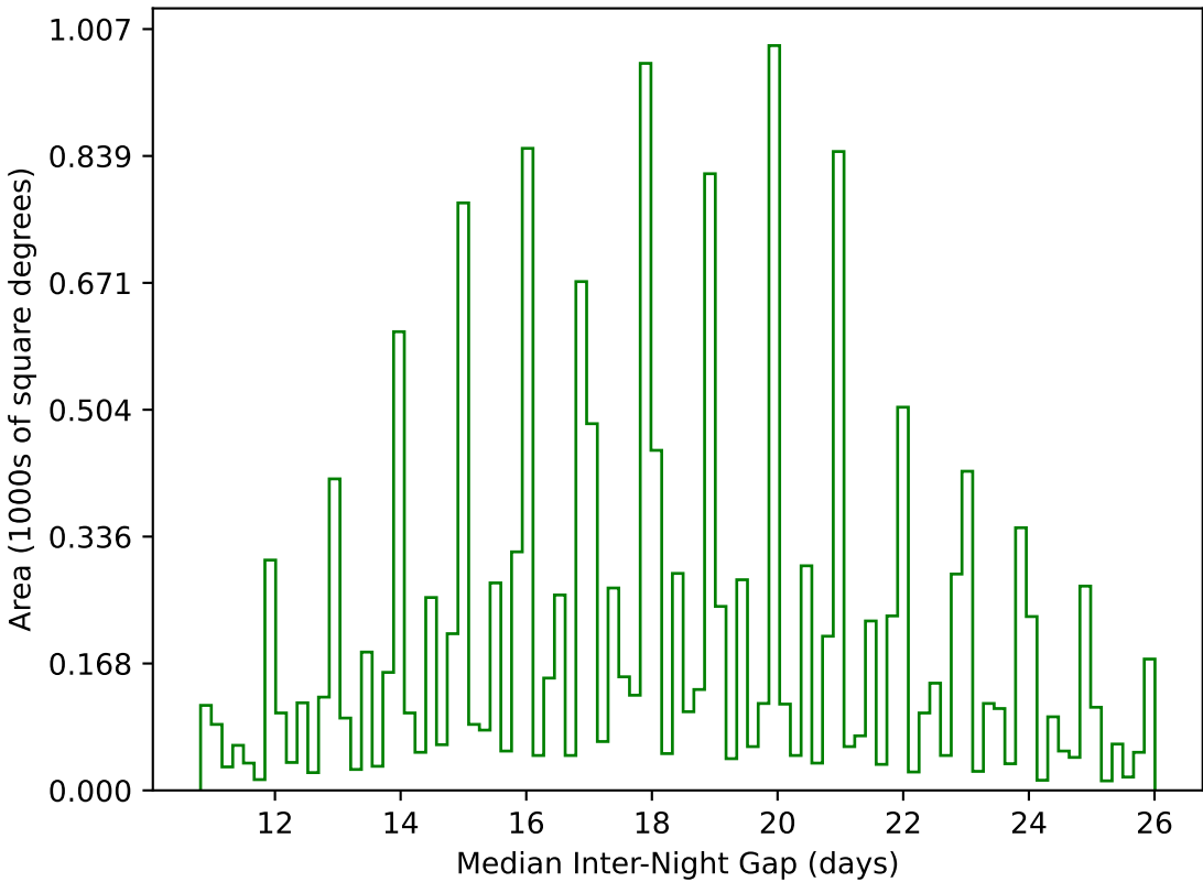
ddf_acor_sf10_lsf15_lsr20_v3.4_10yrs WFD g band: Median Inter-Night Gap
