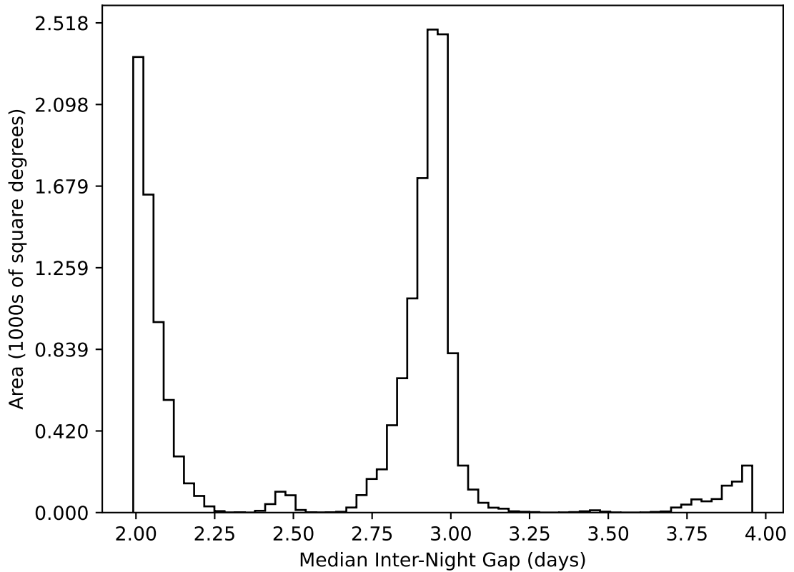
ddf_acor_sf10_lsf15_lsr20_v3.4_10yrs WFD all bands: Median Inter-Night Gap
