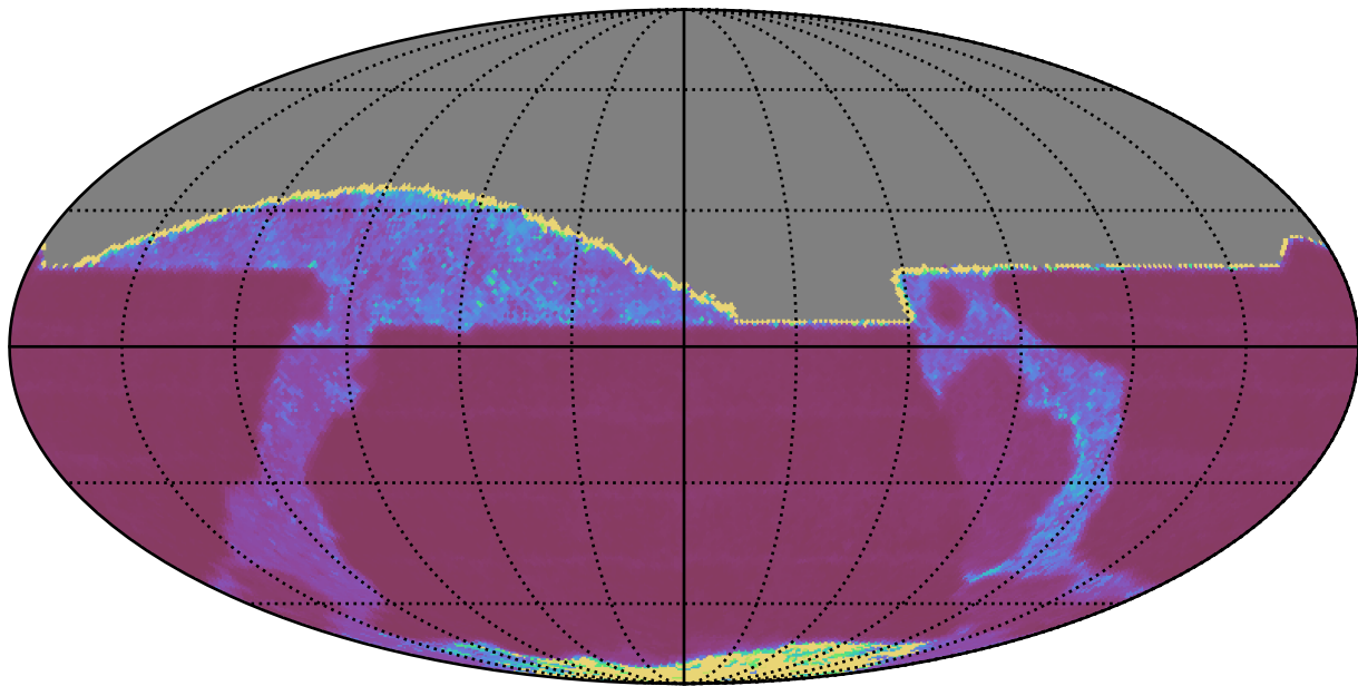
ddf_acor_sf10_lsf15_lsr20_v3.4_10yrs All sky z band: Median Inter-Night Gap
