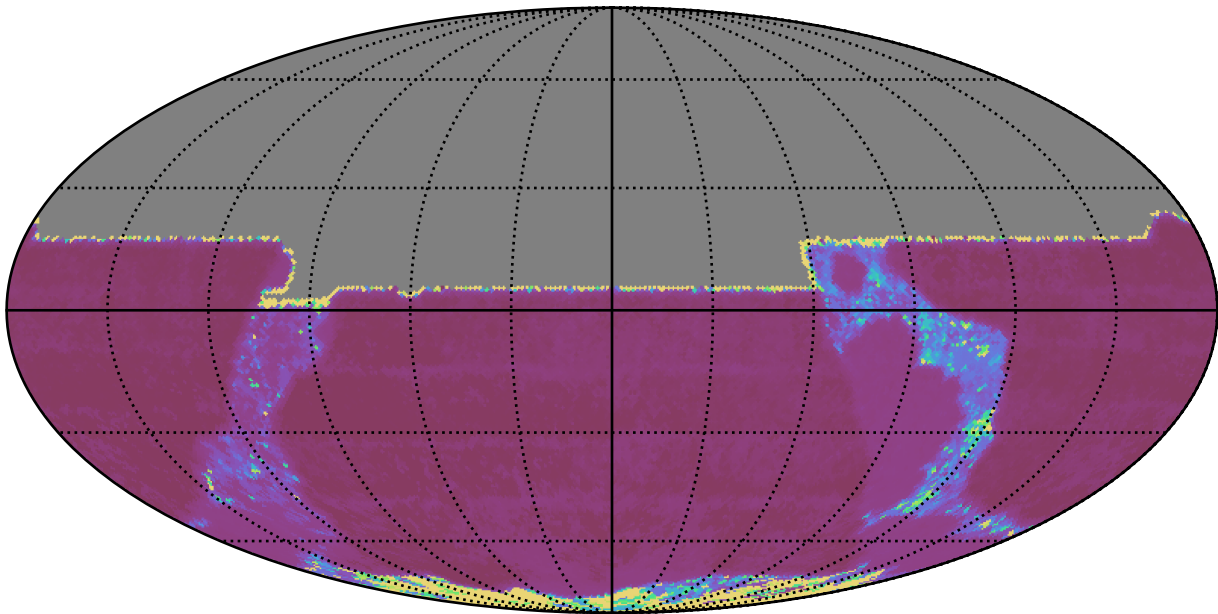
ddf_acor_sf10_lsf15_lsr20_v3.4_10yrs All sky y band: Median Inter-Night Gap
