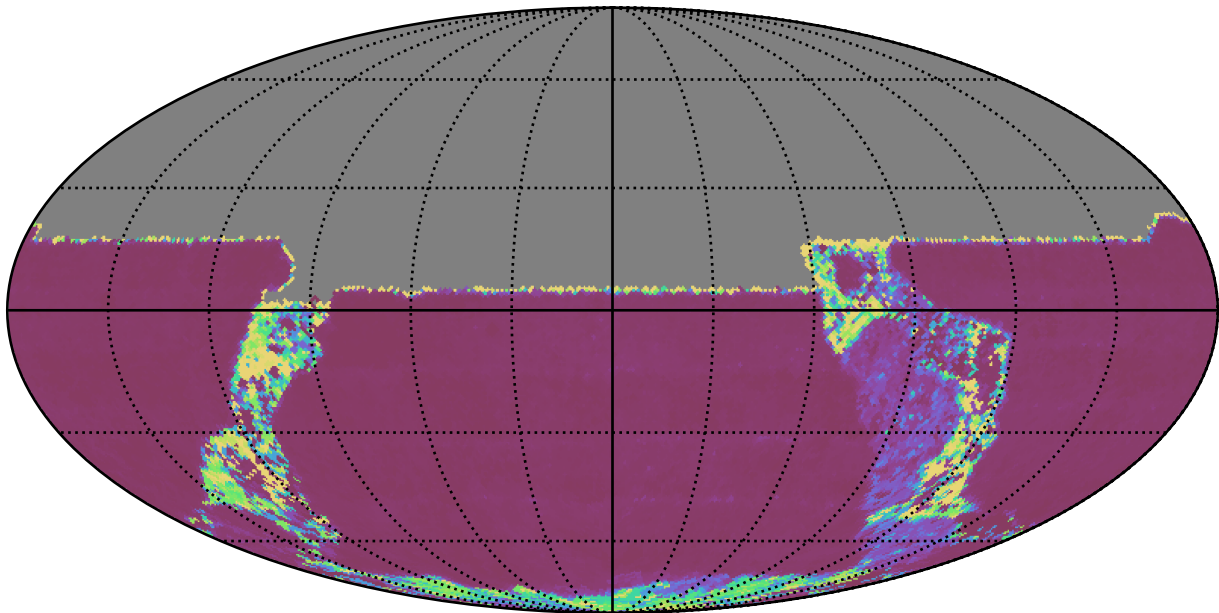
ddf_acor_sf10_lsf15_lsr20_v3.4_10yrs All sky u band: Median Inter-Night Gap
