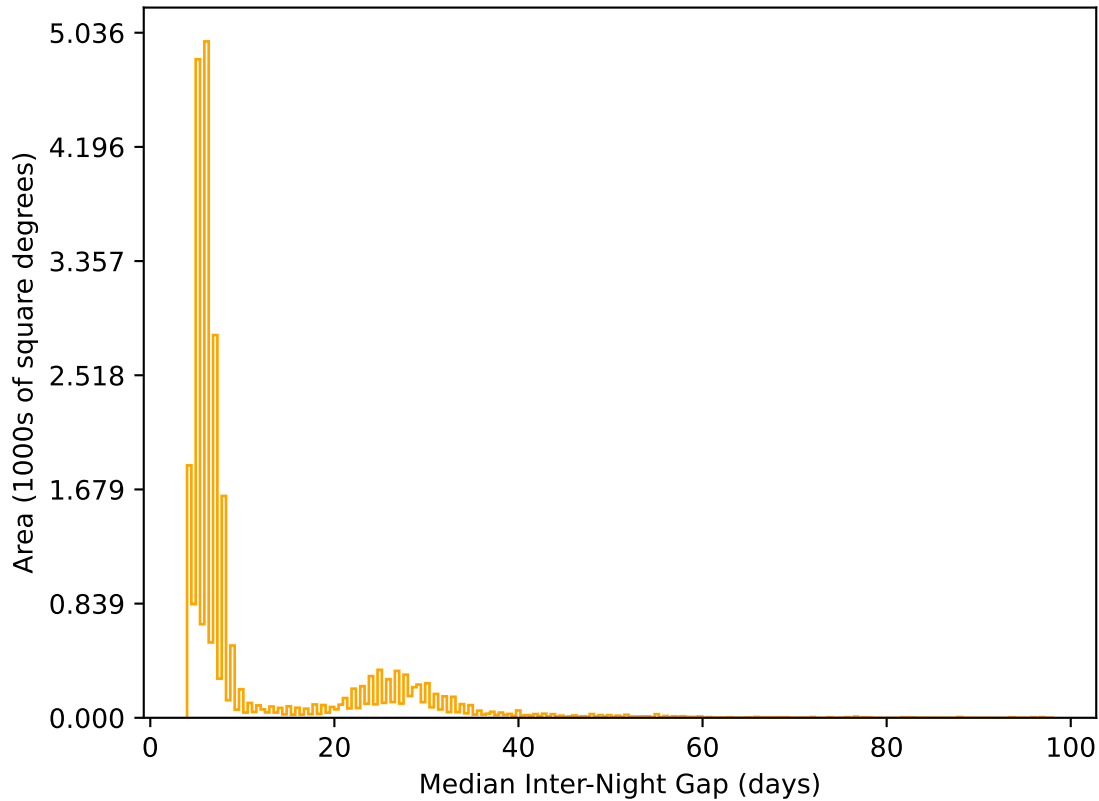
ddf_acor_sf10_lsf15_lsr20_v3.4_10yrs All sky r band: Median Inter-Night Gap
