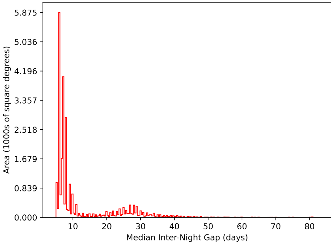
ddf_acor_sf10_lsf15_lsr20_v3.4_10yrs All sky i band: Median Inter-Night Gap
