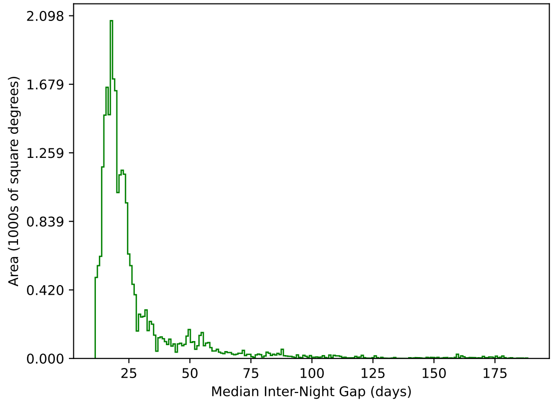
ddf_acor_sf10_lsf15_lsr20_v3.4_10yrs All sky g band: Median Inter-Night Gap
